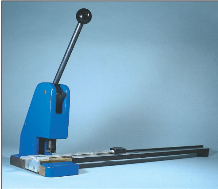
Miters on two ends at the same time. Reversible cutting anvil for long life, and guides for 1/4" and 1/2" width matrix.
