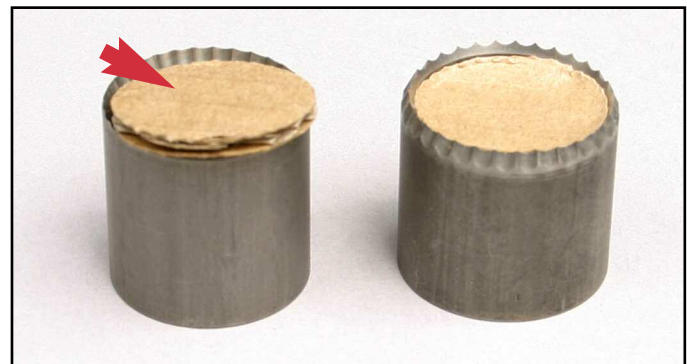
Cuts were made into corrugated using no ejection material, notice the Wagner Inside-Inside Bevel Serrated on the left - the waste does not stay inside the punch, as it does in the conventional outside bevel and center bevel punch as shown on the right.
