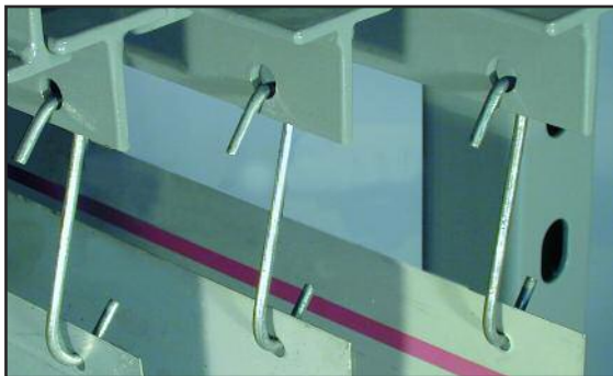
Offset plates hang by "S" hooks (overall length: 2-7/8"). Hanging holes on "T" storage bar are factory-drilled.
