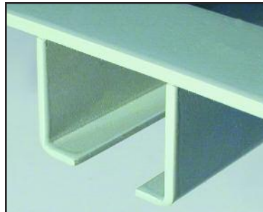
The twin "L" configuration of the Bobst storage rack. Bobst dies slide into the rack between the twin "L's" supported by the two pins.
