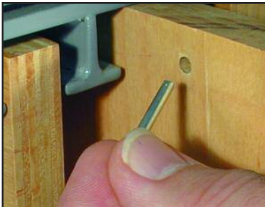
A close-up view of the "T" configuration of rack slides used on Platen storage systems. Dies slide between the channels supported by the two pins.
