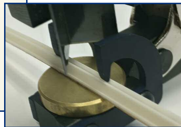
Locator arms hold matrix securely by applicator for secure cutting, 90° blade makes clean, accurate cuts. Brass anvil and 90° cutting blade are replaceable.
